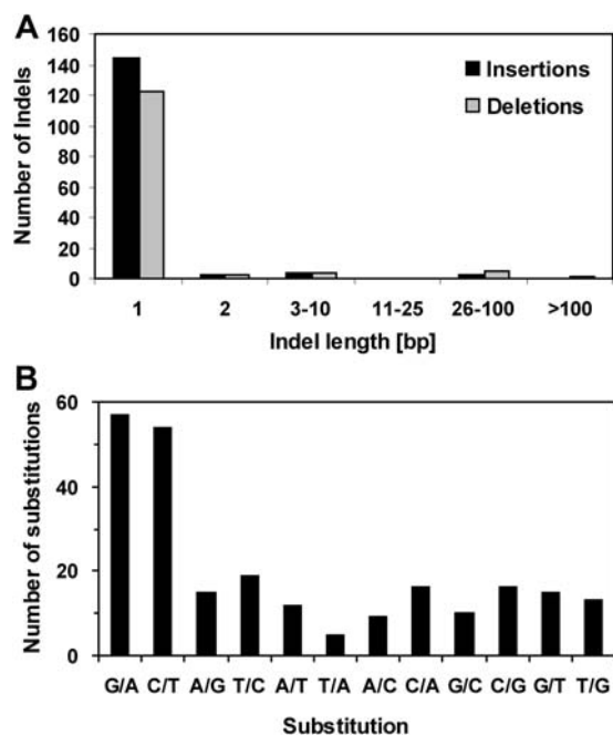
Figure 6. Indel length and nucleotide substitution classes in the 262-kb numtDNA of Arabidopsis. A, Indel length classes in the numtDNA. Indels of specified length were pooled into the six groups shown on the x axis. Histograms indicate the number of insertions or deletions. Insertions are nucleotides present in the numtDNA but absent in the Arabidopsis mtDNA. Deletions are nucleotides absent in the numtDNA but present in the Arabidopsis mtDNA. B, Frequency of 12 types of nucleotide substitution in the numtDNA relative to mtDNA (e.g. G/A indicates that G is present in mtDNA and A is present in the nuclear copy).
